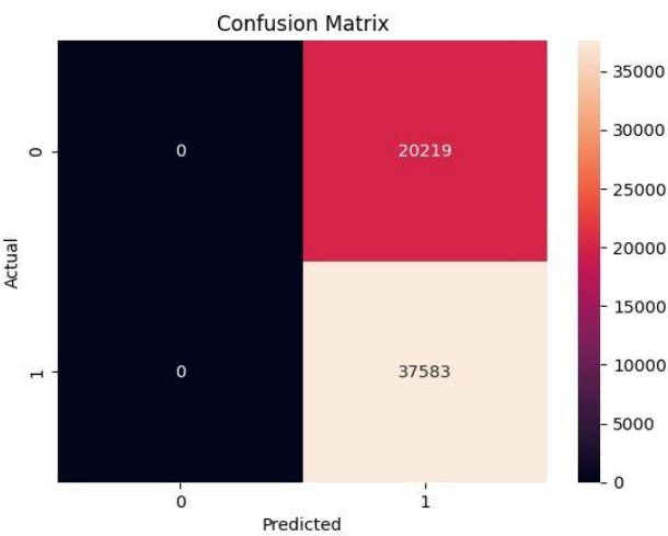
Figure 4. Confusion matrix showing classification performance of the proposed model.
